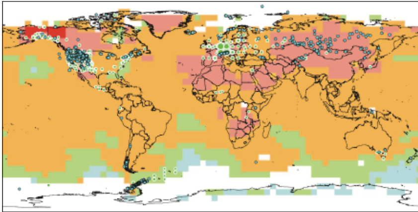
Figure 3 Bernstein et al., 2007
