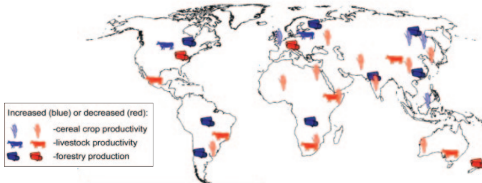
Figure 1 Easterling et al. 2007, 302 6
