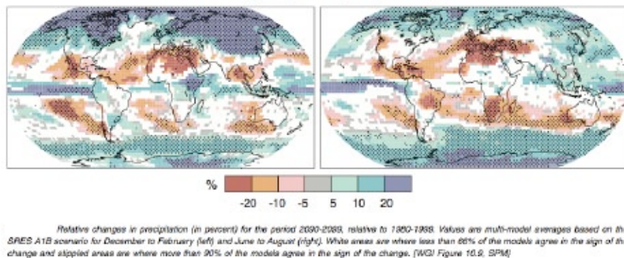
Figure 1 Bernstein et al., 2007
